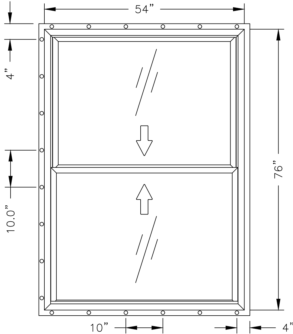
6000 Tilt Double Hung WINDOW – FIN INSTALLATION MAXIMUM SIZE 54" X 76" DESIGN PRESSURE +/- 55 PSF MISSILE D – WIND ZONE 3
